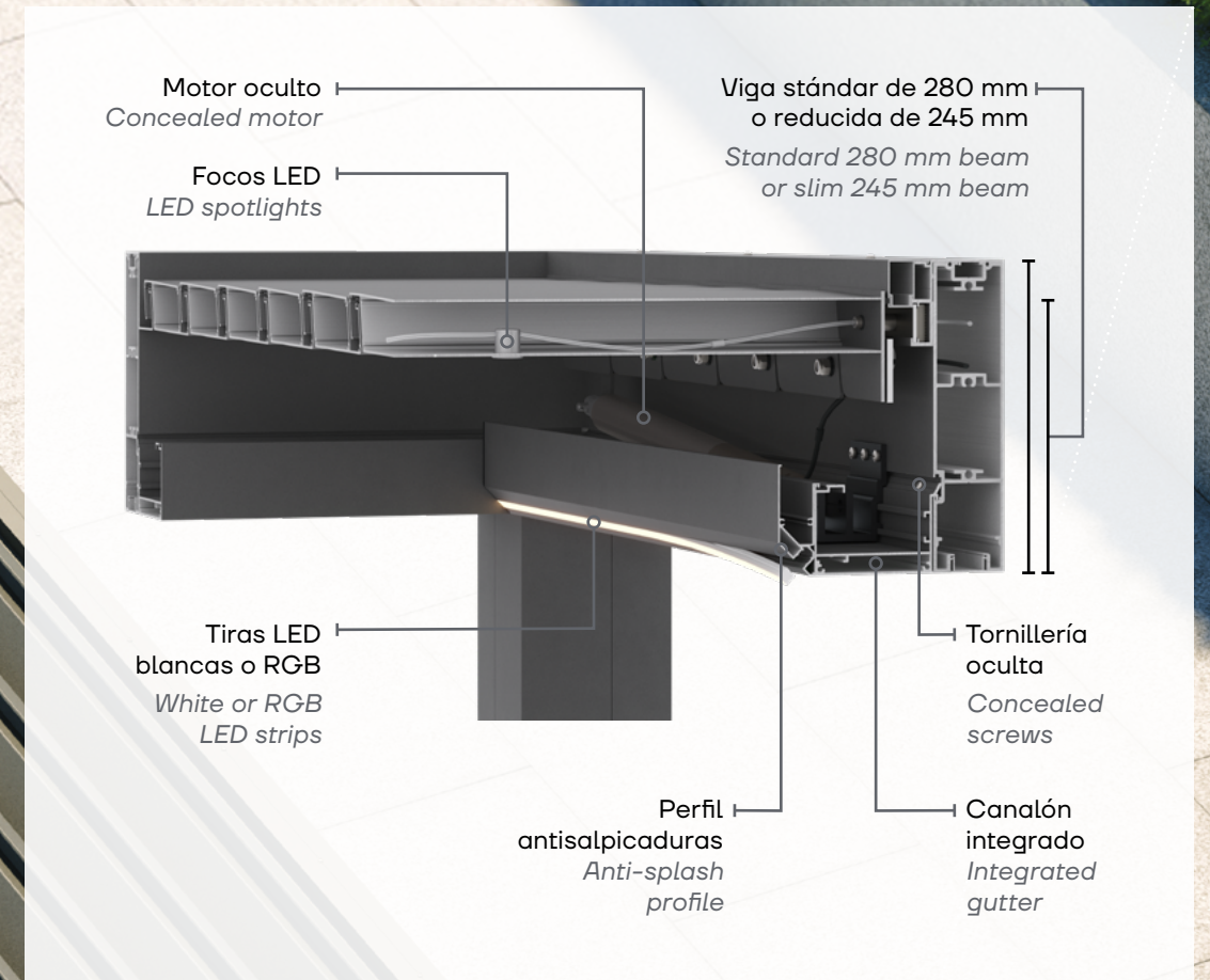
Detalle interior de pérgola Pergola interior detail
