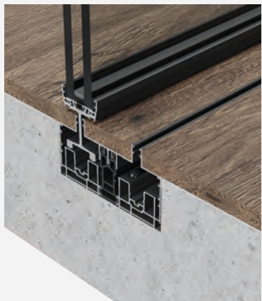
Flush threshold Floor finish
