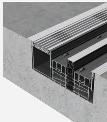
Drainage channel with aluminium gutter
